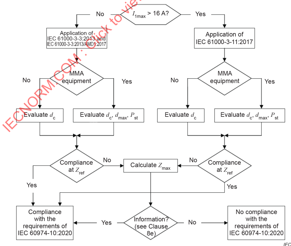
Figure 6 – Overview of flicker requirements
