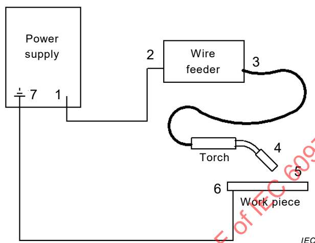
Figure B.1 – Example of MIG/MAG equipment
