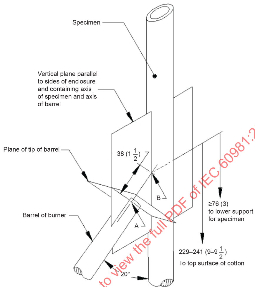
Figure 6 – Essential dimensions for flame test
