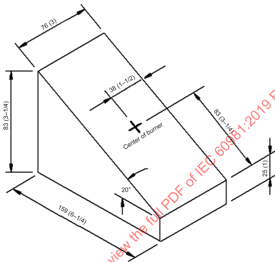
Figure 5 – Dimensions of wedge
