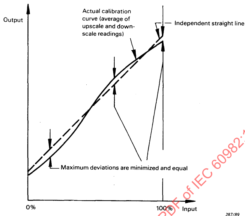
Figure 10 - Linearity
