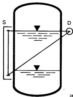
Figure 4 - Line source and point detector
