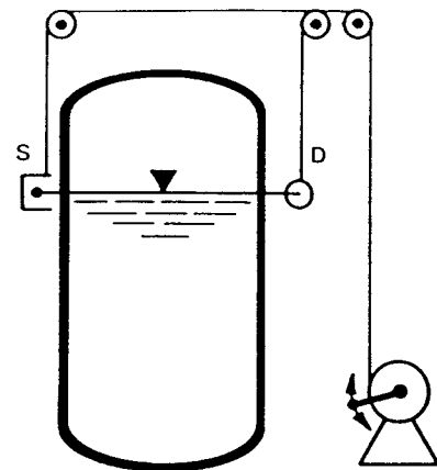
Figure 5 - Point source and point detector continuously following the level
