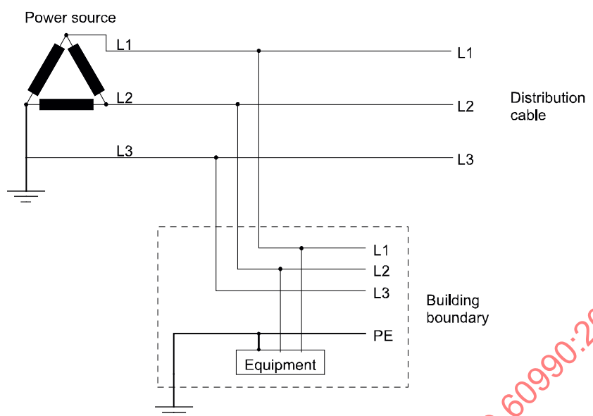
Figure I.6 – Example of 3-line TT power system
