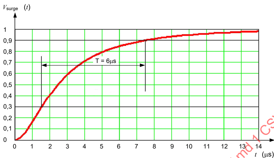
Figure E.8 – Voltage surge (10/700 \mu s): rise time response T
