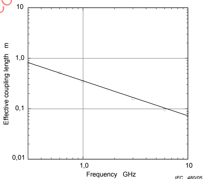
Figure 6 – Effective coupling length for a 1 m metallic cable
