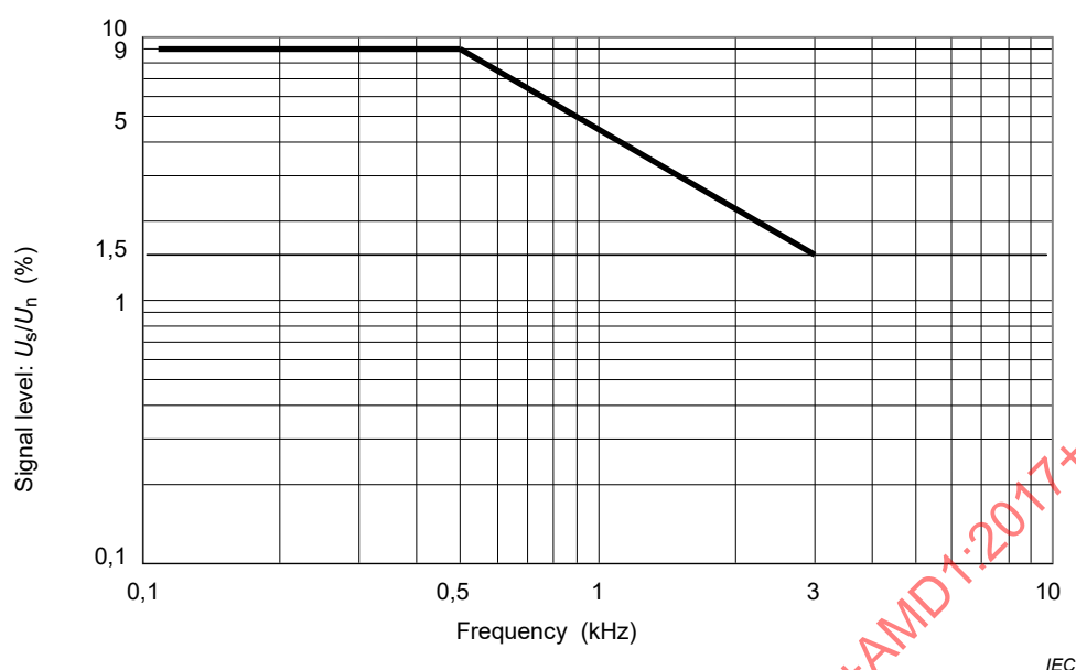
Figure 3 – Meister curve for ripple control systems in public networks (110 Hz to 3 000 Hz)
