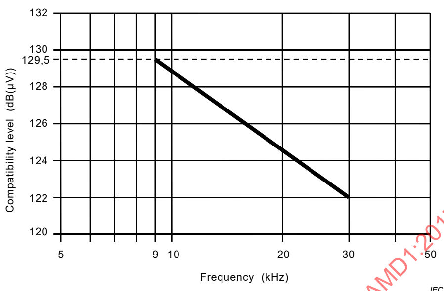
Figure C.2 – Compatibility levels for voltage distortion in differential mode from 9 kHz to 30 kHz
