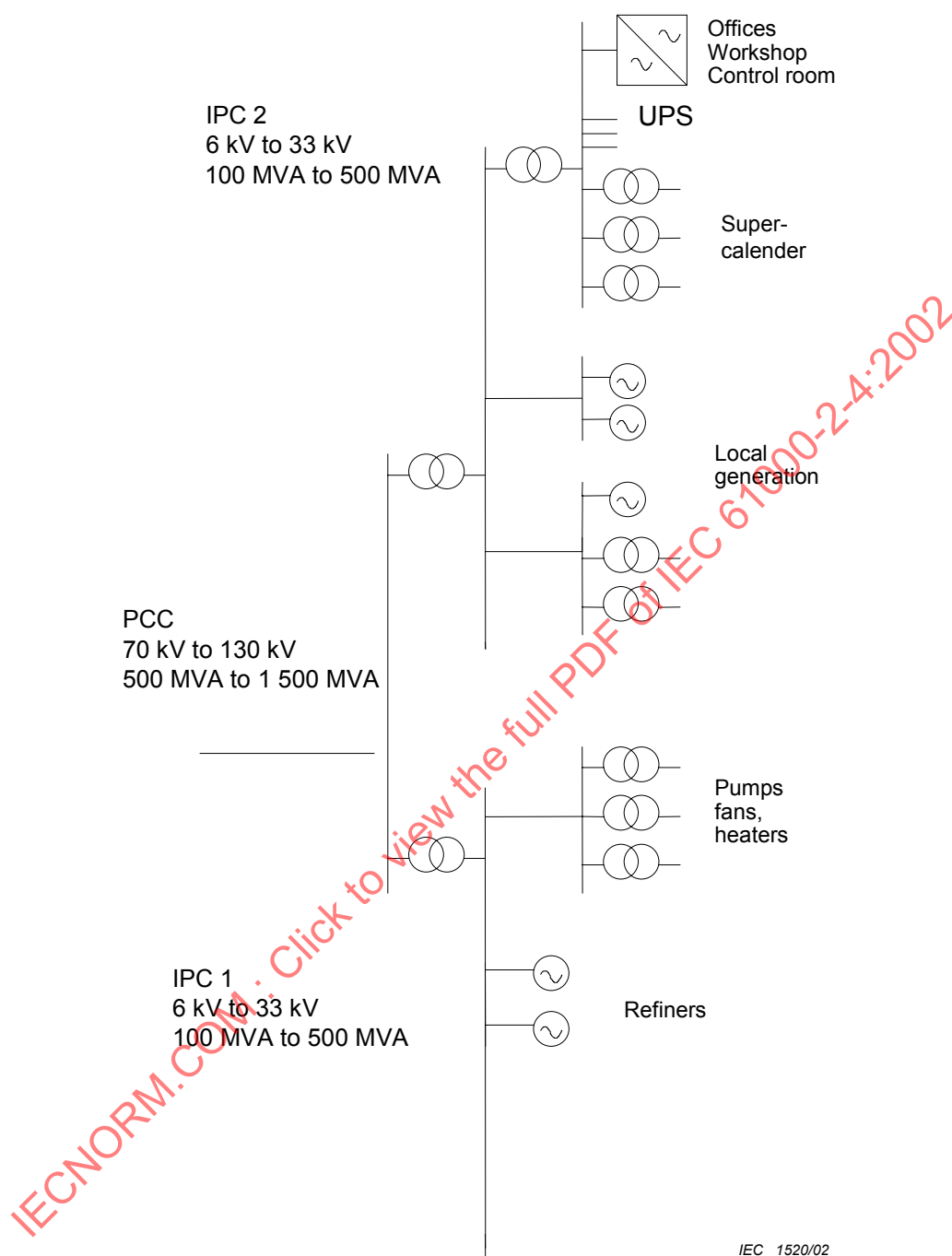
Figure B.2 – Example of power distribution in the paper industry
