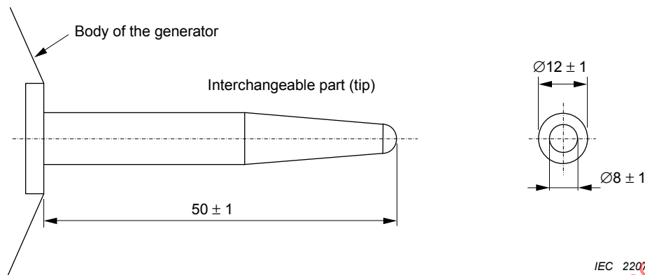
3a) – Discharge electrode for air discharges
