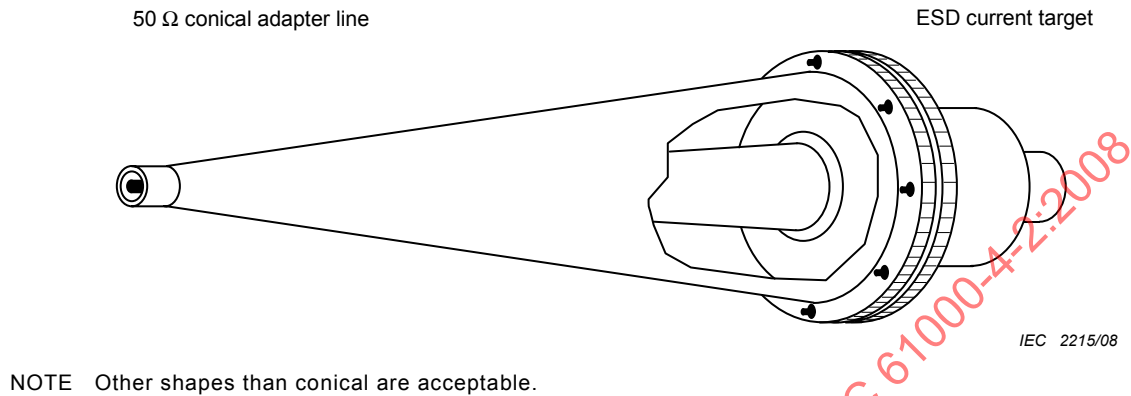
Figure B.1 – Example of a target adapter line attached to current target
