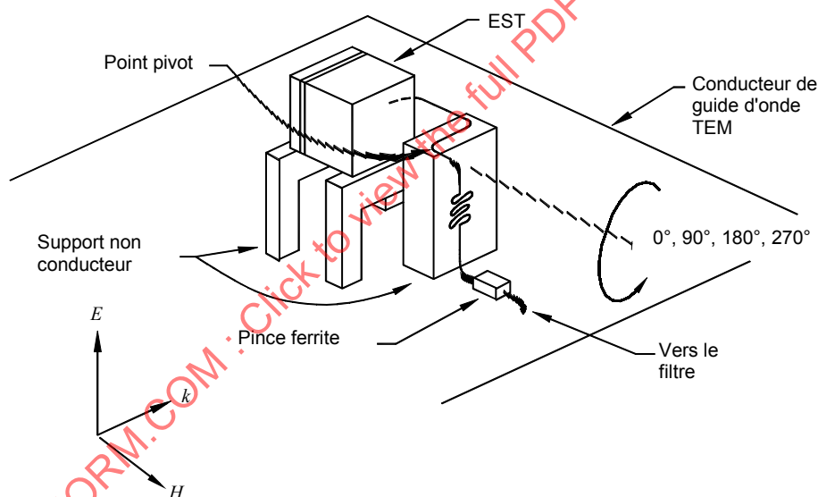
Figure B.1a – Polarisation verticale
