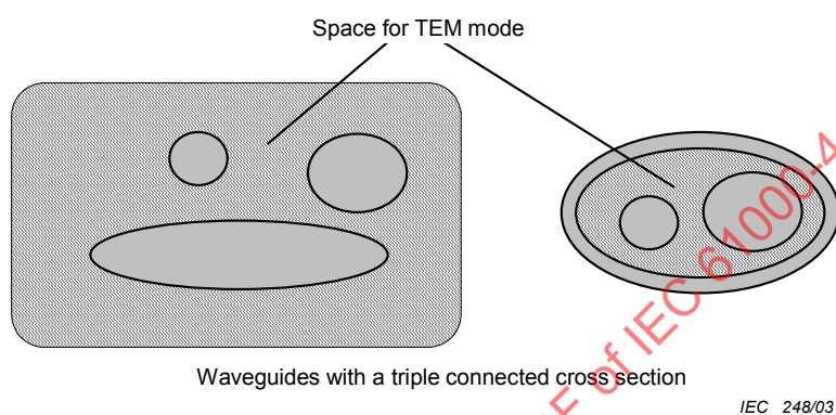
Figure D.2 – Example waveguides for TEM-mode propagation
