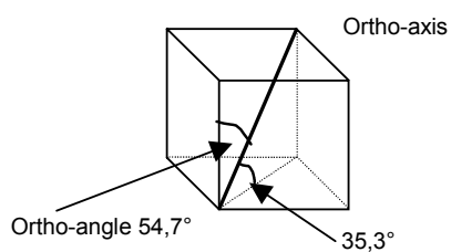
Figure A.2a – The ortho-axis and the ortho-angle
