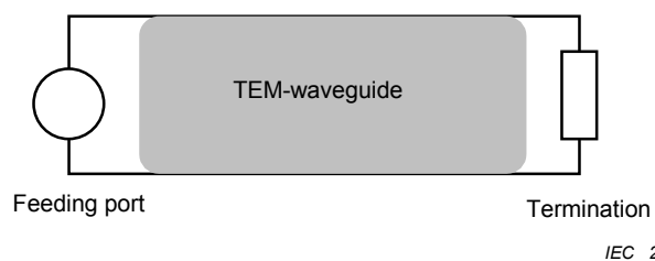
Figure D.4 – Transmission line model for TEM propagation
