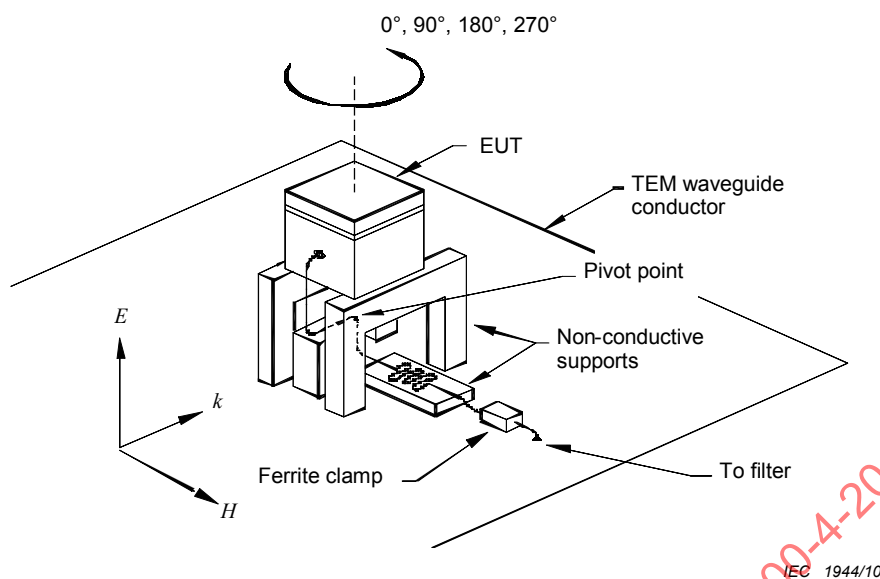
Figure B.1a – Vertical polarization
