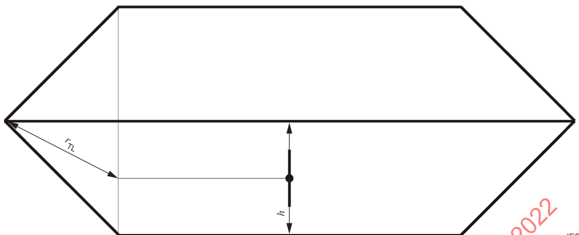
a) Two-port TEM cell
