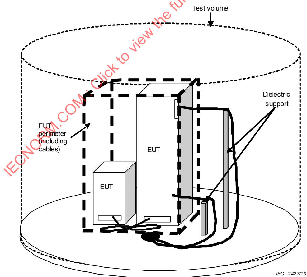
Figure 8 – Example test set-up for floor-standing equipment
