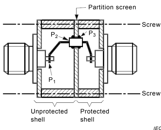
c) Example of a test fixture with a DUT in a feed-through configuration
