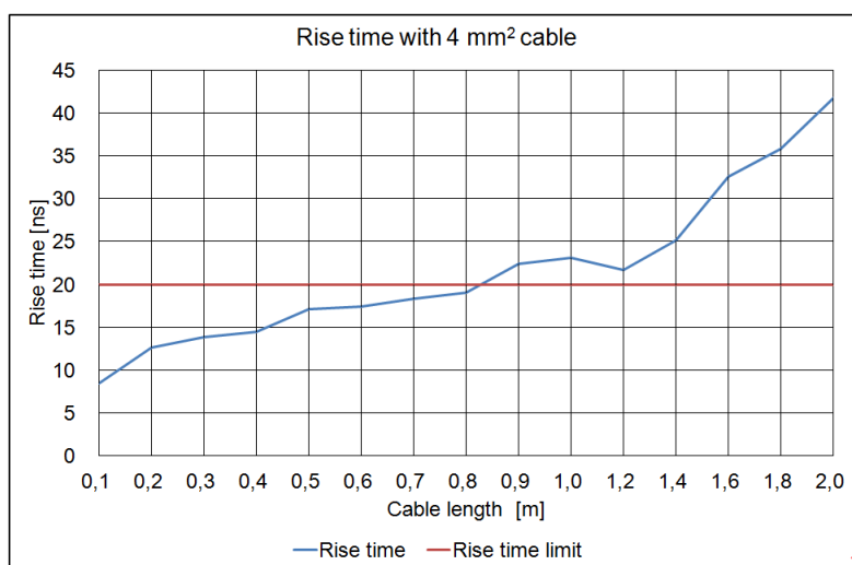
Figure A.6 – Rise time calibration results with 4 mm² cables
