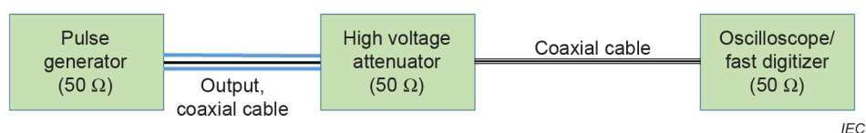
(b) Configuration of verification for test level in voltage
