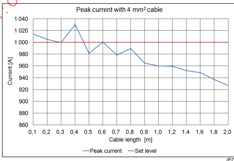
Figure A.5 – Peak current calibration results with 4 mm² cables: 1 000 A ± 8 %
