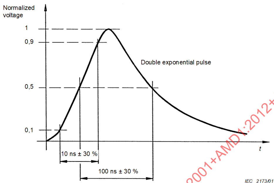
Figure C.5 – Waveshape of an EC11 pulse into a 50 \Omega load
