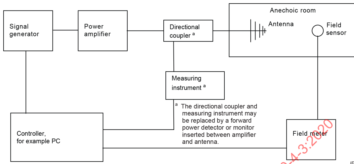
Figure 6 – Measuring setup
