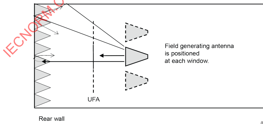
Figure C.2 – Most of the reflected waves are eliminated (applies for top and side view)
