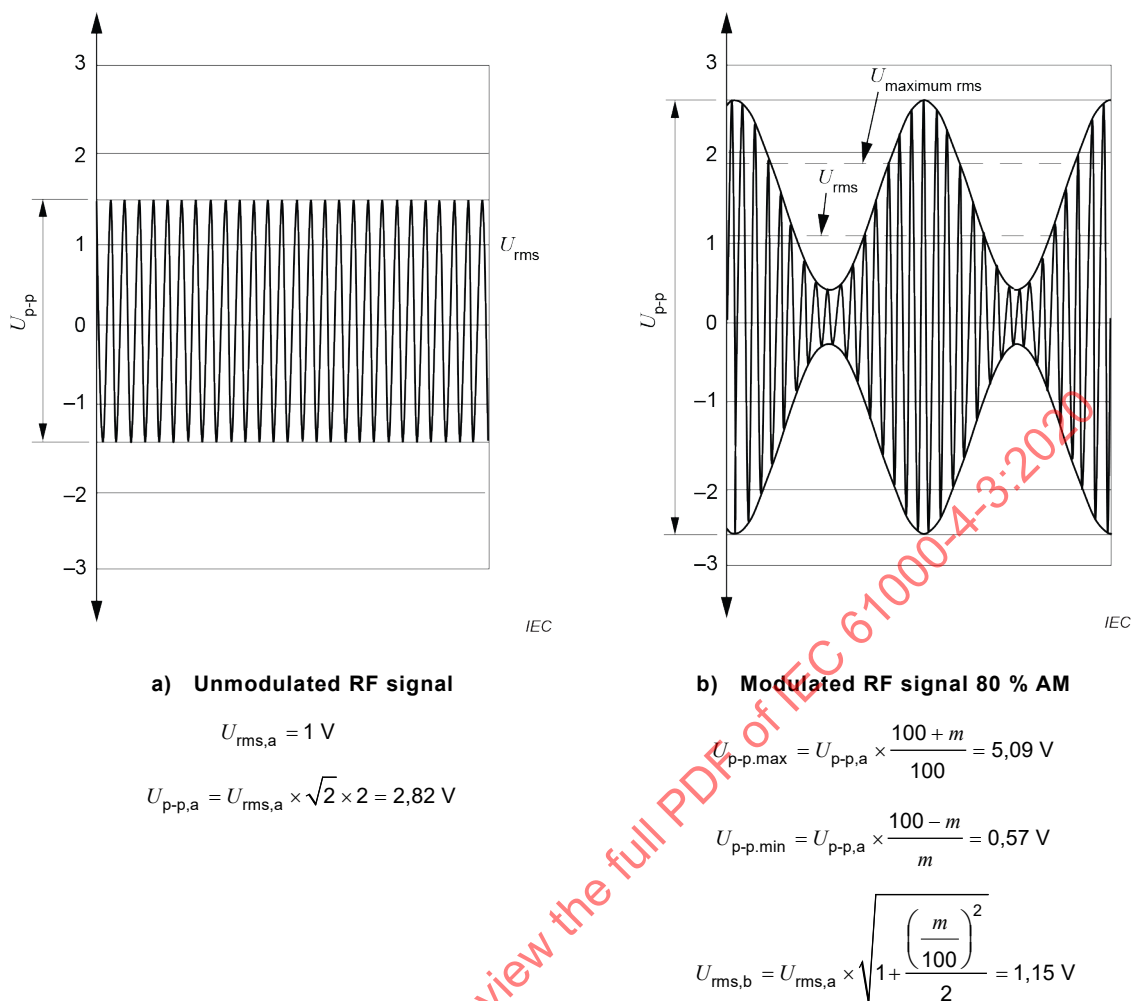
Figure 1 – Definition of the 80 % amplitude modulated (AM) test signal and the waveshapes occurring
