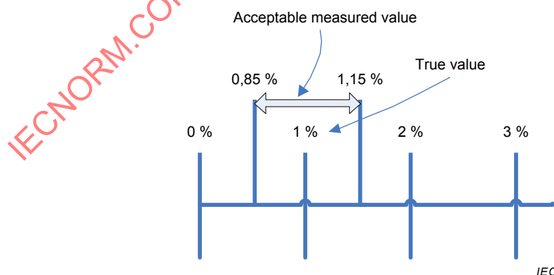
Figure 5 – Example of supply voltage unbalance uncertainty
