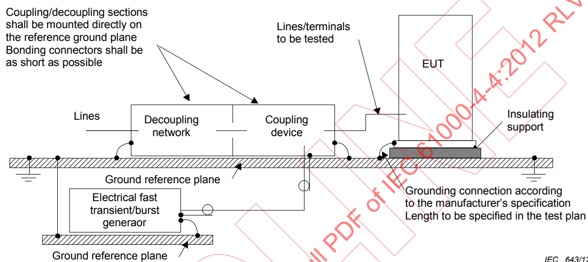
Figure 9 – Block diagram for electrical fast transient/burst immunity test
