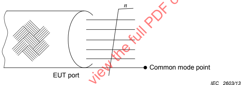
b) Definition of a common mode point with screened cables
