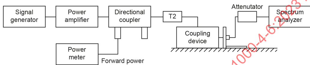
Figure J.1 – Amplifier linearity measurement setup
