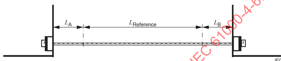
Figure A.4 – Test jig
