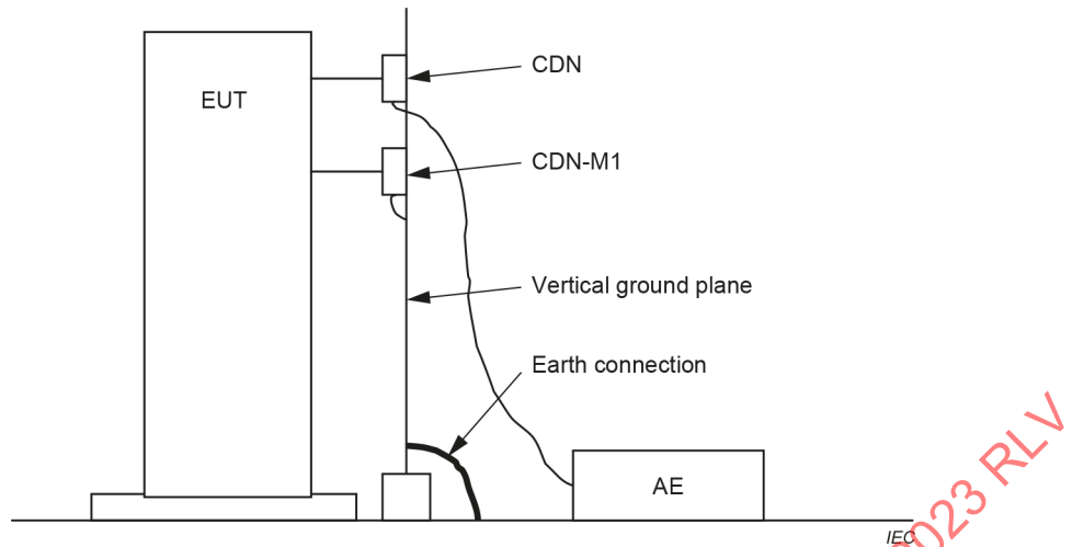
Figure F.2 – Example of large EUT test setup with vertical reference ground plane
