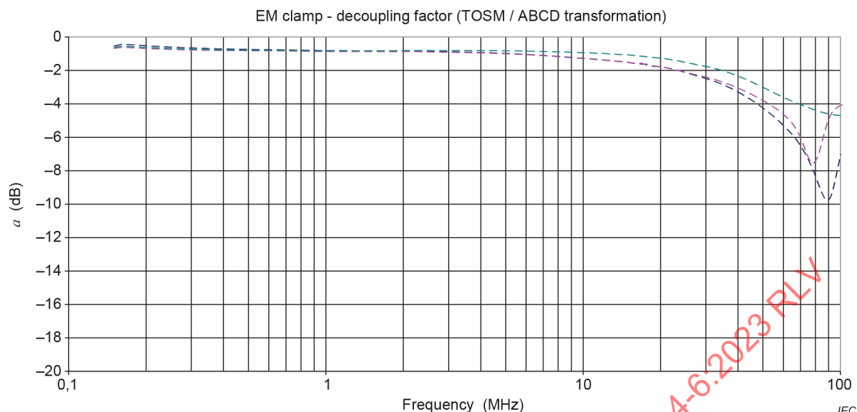
Figure A.8 – Typical examples for decoupling factors, three typical clamps
