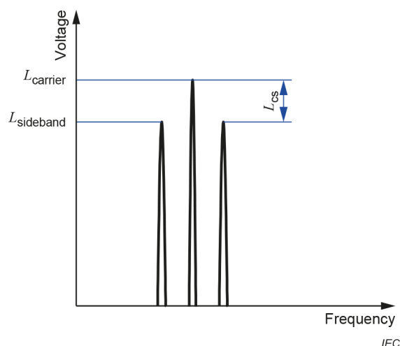
Figure J.4 – Spectrum of AM modulated signal
