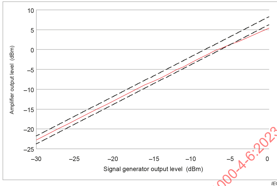
Figure J.2 – Linearity characteristic
