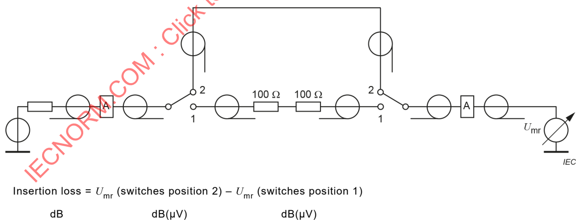
Figure 13 – Setup principle for measuring the insertion loss of two 150 Ω to 50 Ω adapters
