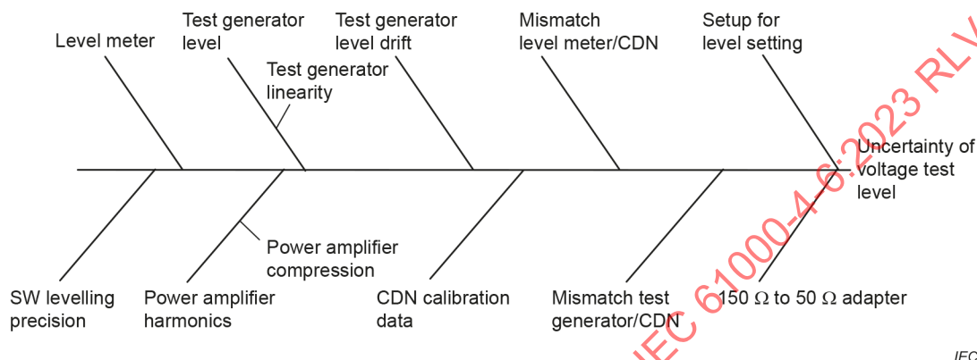
Figure G.1 – Example of influences upon voltage test level using CDN
