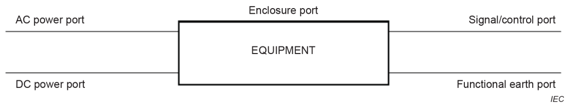
Figure 3 – Ports of an apparatus or facility
