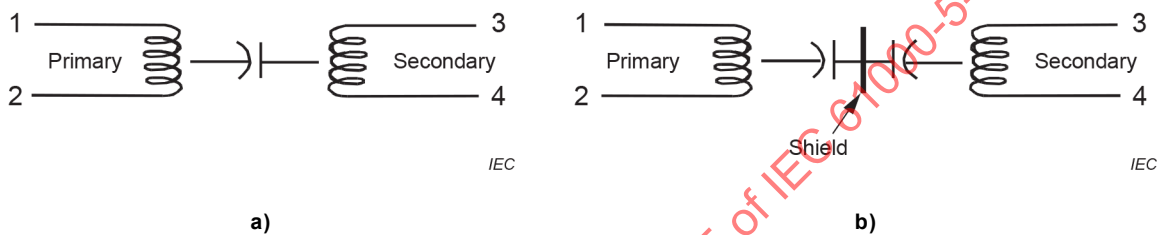
Figure 18 – Propagation of a 0,5 μs to 100 kHz ring wave operating in the differential mode through a "line isolator" transformer
