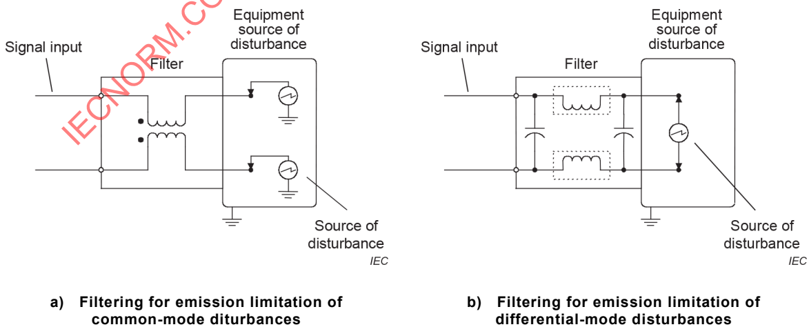
Figure 10 – Prevention of interference on installed equipment
