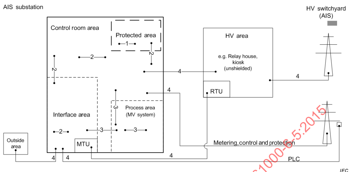
AIS substation
