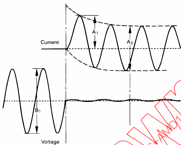
Figure 10 – Example of calibration record for short-circuit test
