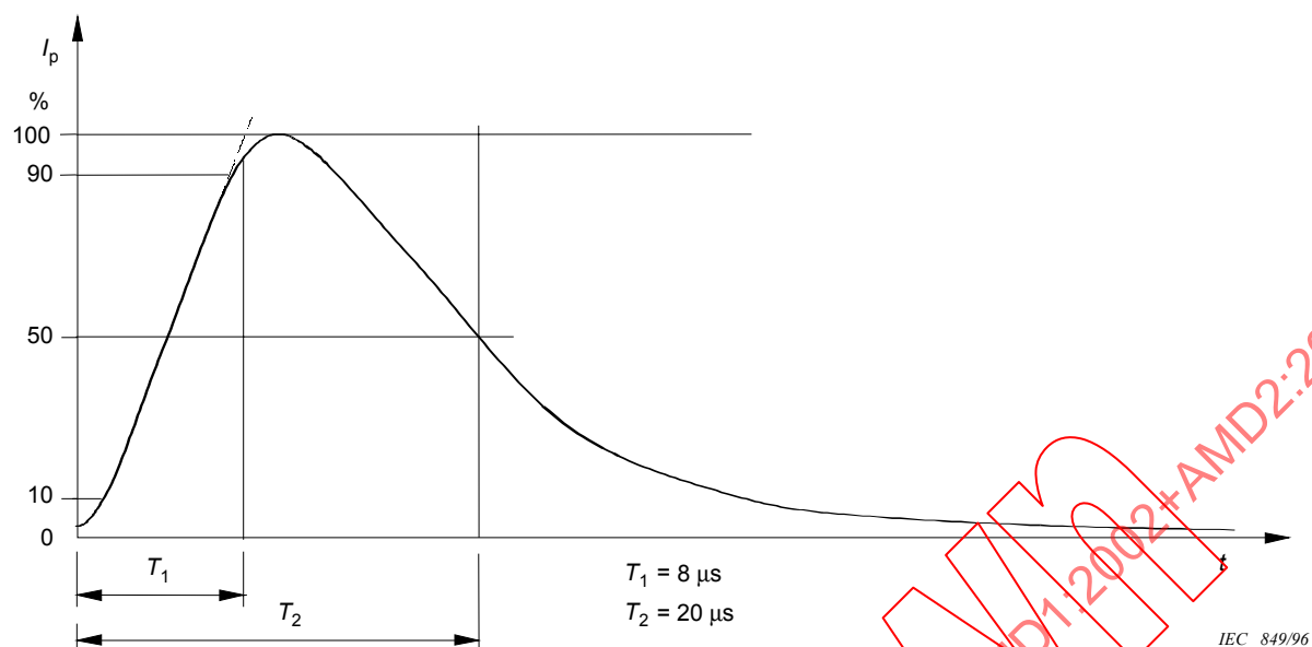
Figure 25 – Onde de courant 8/20 \mu\text{s}
