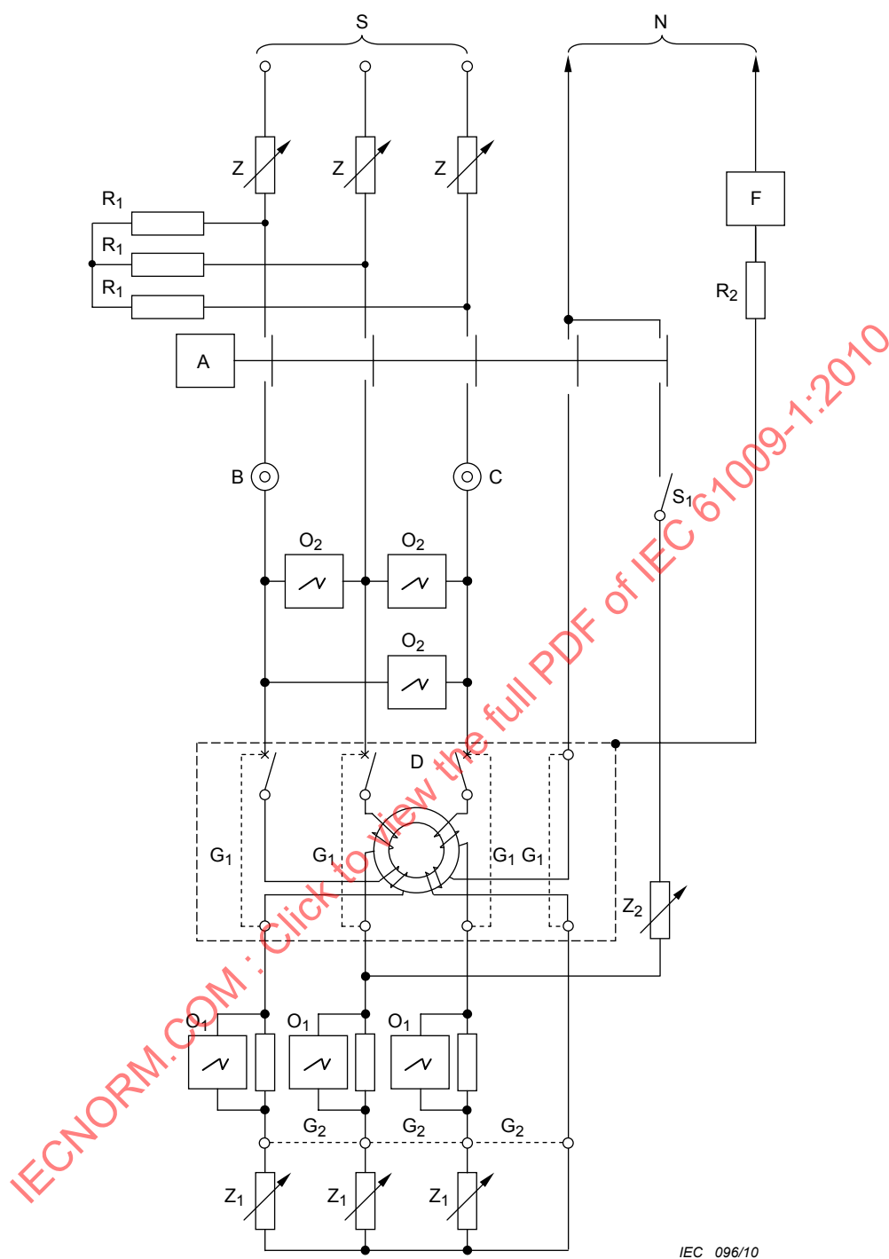
Figure 11 – Test circuit for the verification of the rated short-circuit capacity of a three-pole RCBO with four current paths on a three-phase circuit with neutral (9.12)
