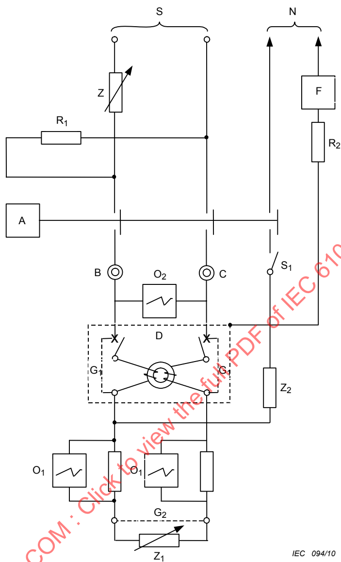
Figure 9 – Test circuit for the verification of the rated short-circuit capacity of a two-pole RCBO, in case of a single-phase circuit (9.12)
