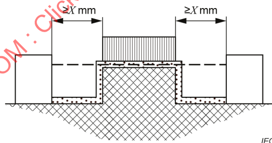
Figure B.5 – Measuring creepage distances and clearances: Example 5
