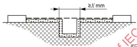
Figure B.1 – Measuring creepage distances and clearances: Example 1
