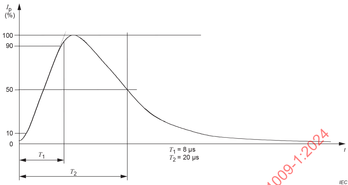
Figure 18 – Surge current impulse 8/20 \mu\text{s}
