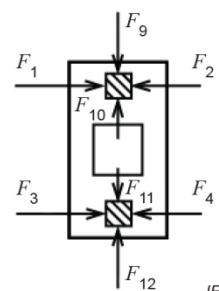
Figure 9 – Application of forces and torques for 4.8.1
