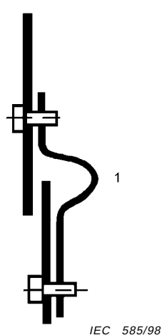
1 Flexible metal strapping bridging
