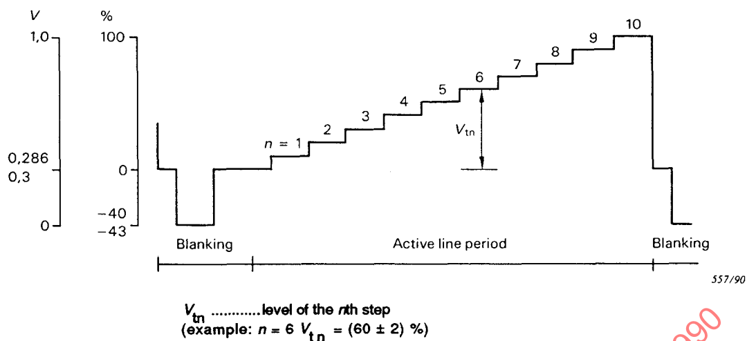
Figure 5 - Test signal for luminance non-linear distortion (10 steps) (clause 2.4)
