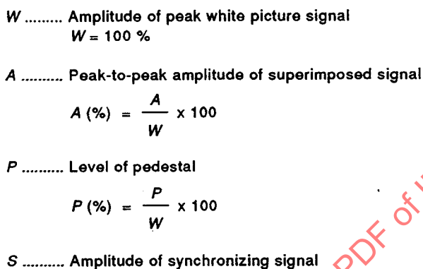
Figure 1 - Video test signal: nominal values, horizontal line
