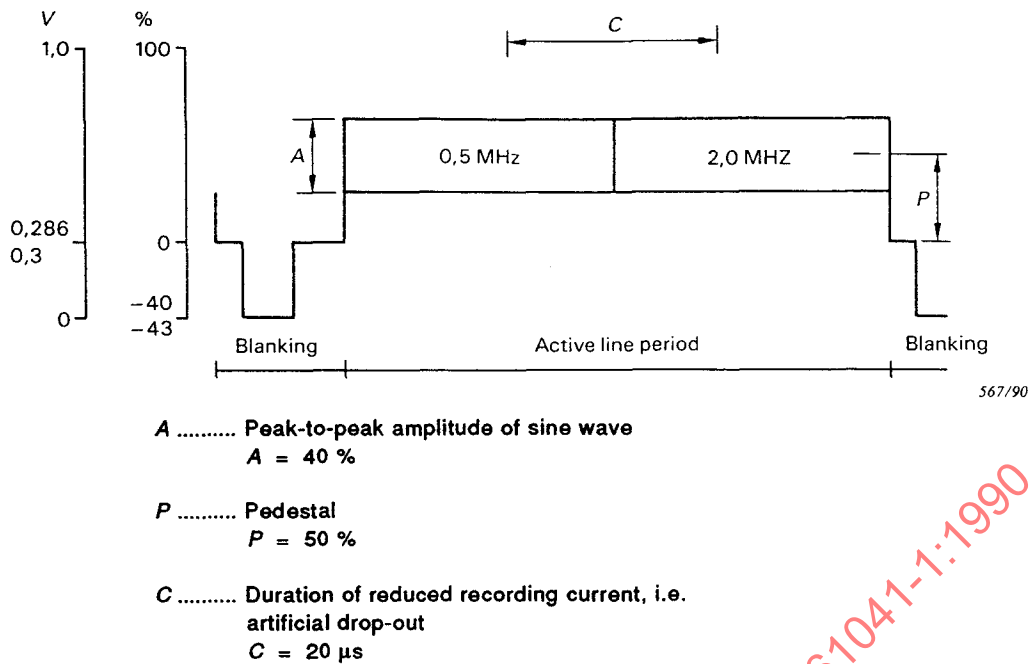
Figure 11b - Test signal for luminance drop-out compensation (to be recorded on the special test tape)
