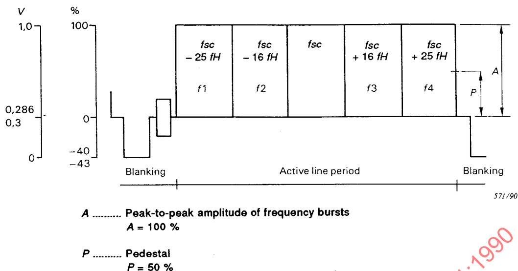
Figure 12 - Test signal for chrominance amplitude/frequency response
