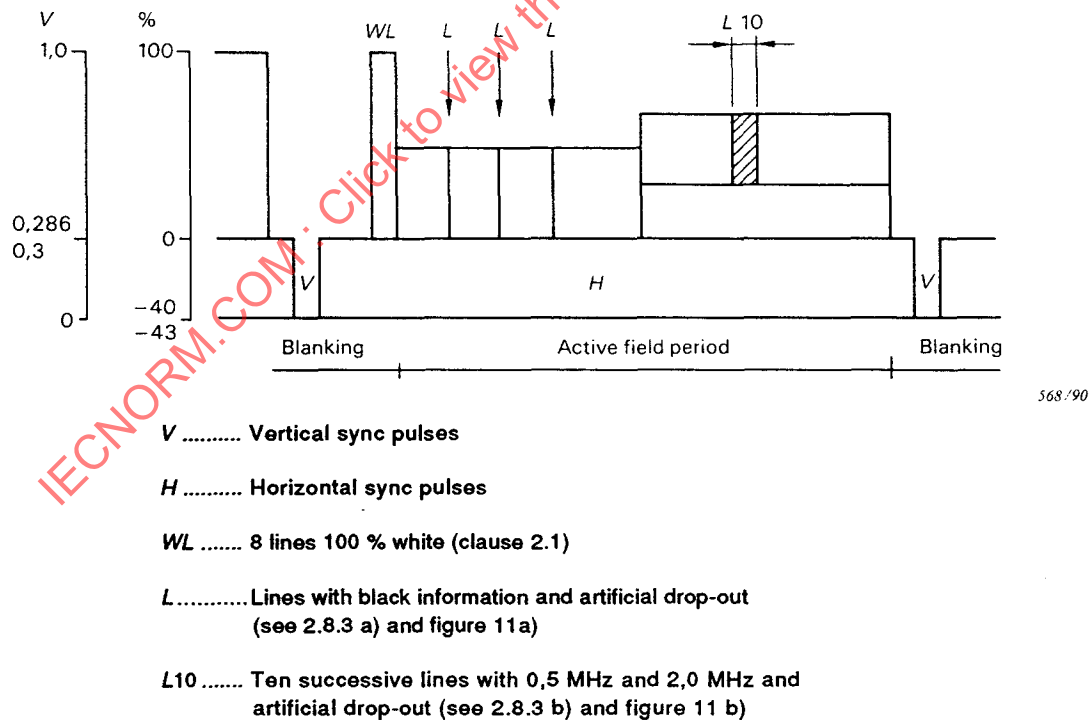
Figure 11c - Test signal for luminance drop-out compensation (to be recorded on the special test tape)
