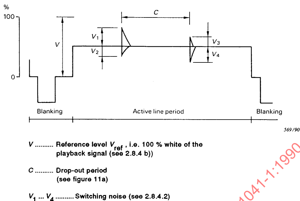
Figure 11d - Drop-out compensation switching noise
