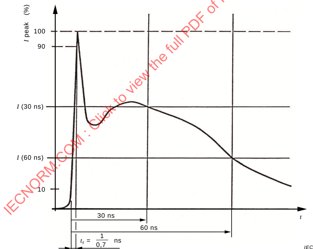
Figure B.4 – Shape of pulse type 3
