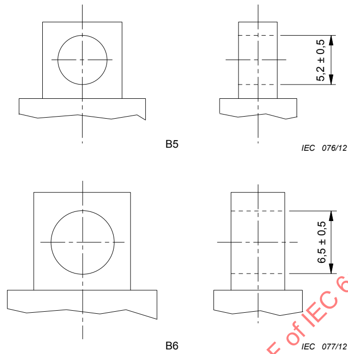
Figure 4 – B-contacts (bolt and nut system)
