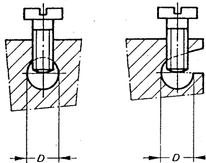
1a - Bornes sans plaquettes Terminals without pressure plates
