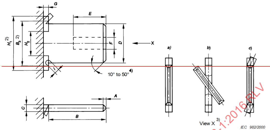
Dimensions of tabs 5)
