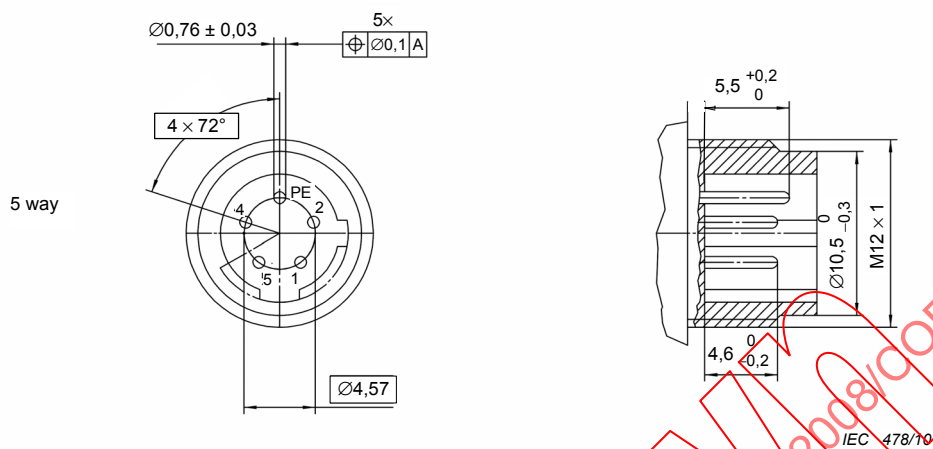
Figure 27 – Pin front view 5 way with C-coding
