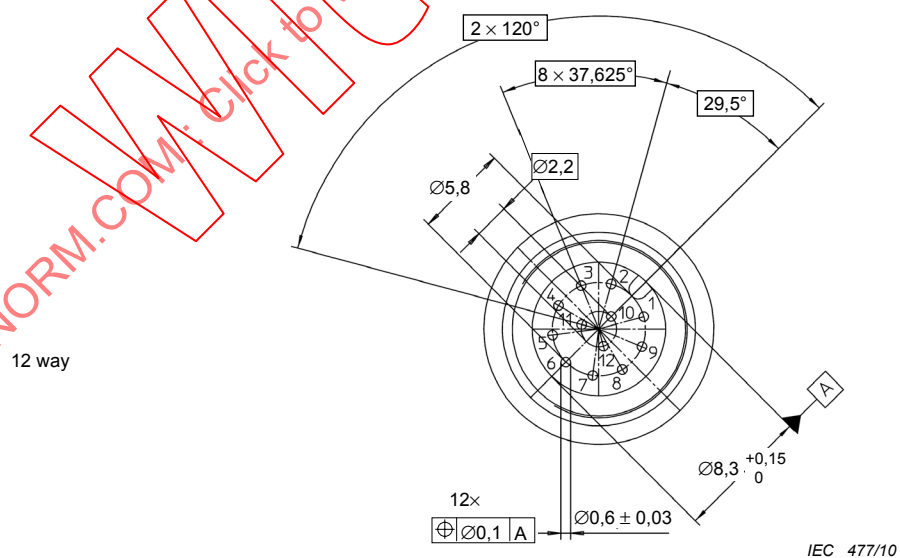
Figure 21 – Pin front view A-coding
