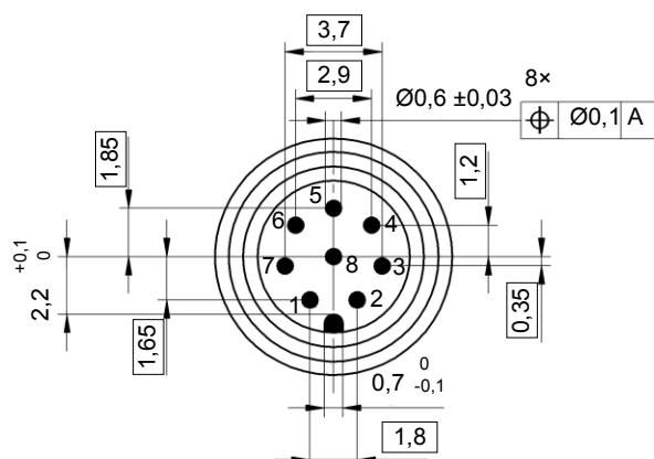
Figure 16 – Pin front view A-coding
