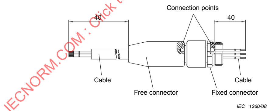
Figure 13 – Contact resistance arrangement
