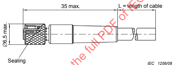
Figure 8 – Non-rewireable connector, female contacts, straight version, with locking nut
