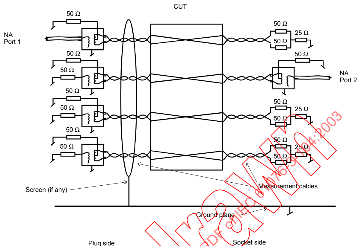
Figure I.2 – FEXT measurement differential and common mode terminations
