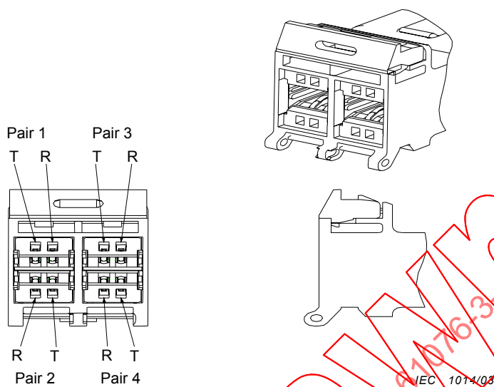
Figure 2 – Fixed connector
