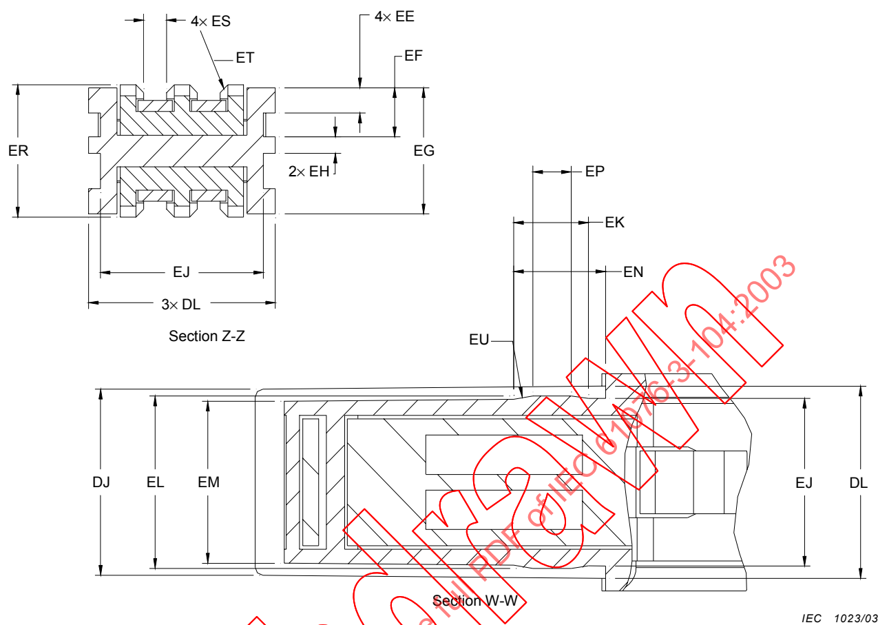
Figure 11 – Variant 04 drawing 2
