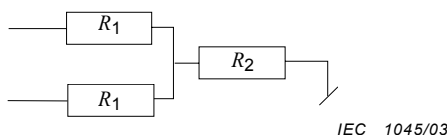
Figure E.3 – Resistor load
