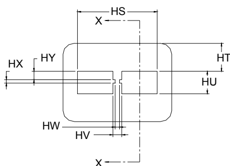
Figure 23 – Free connector location GO gauge
