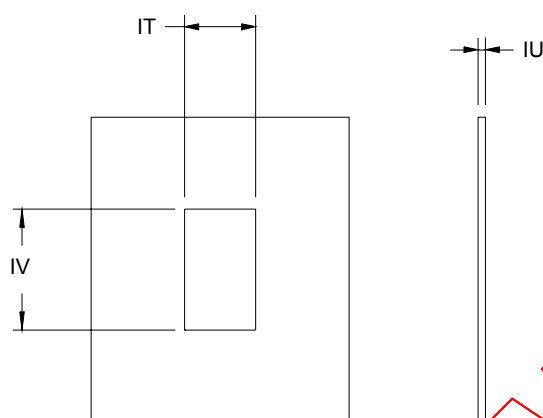
Figure 27 – Test panels
