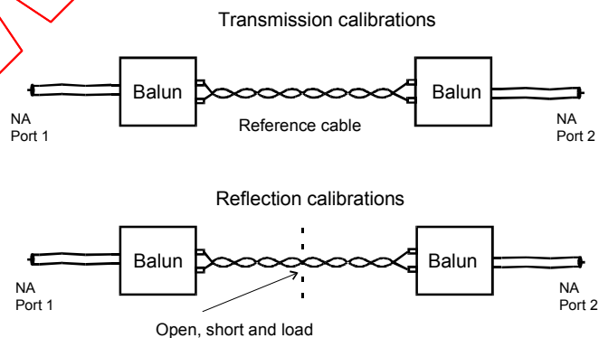
Figure F.1 – Calibration
