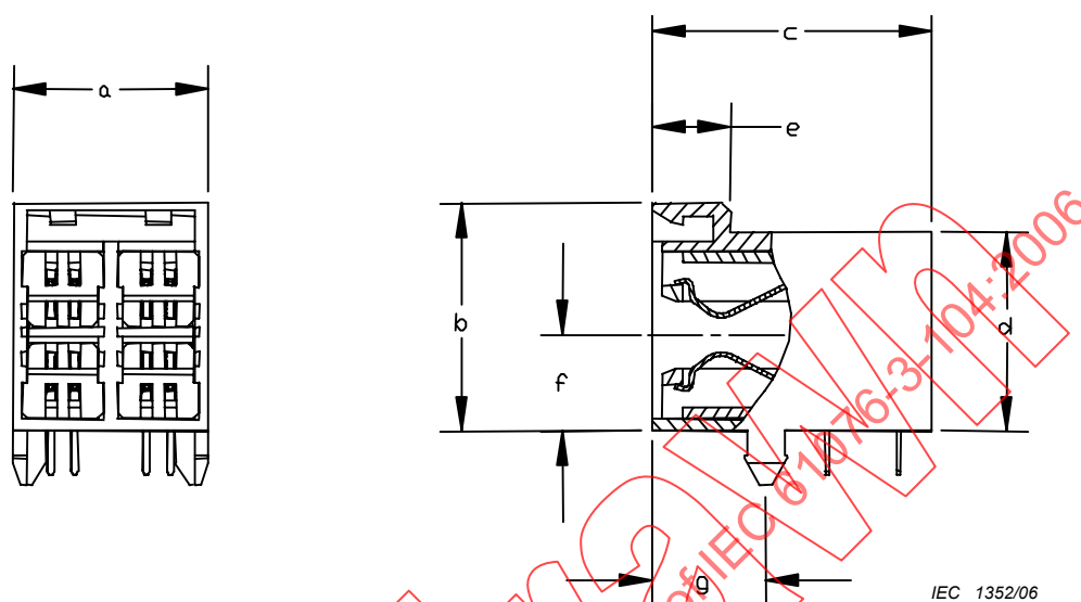
Figure 5 – Variant 02 drawing
