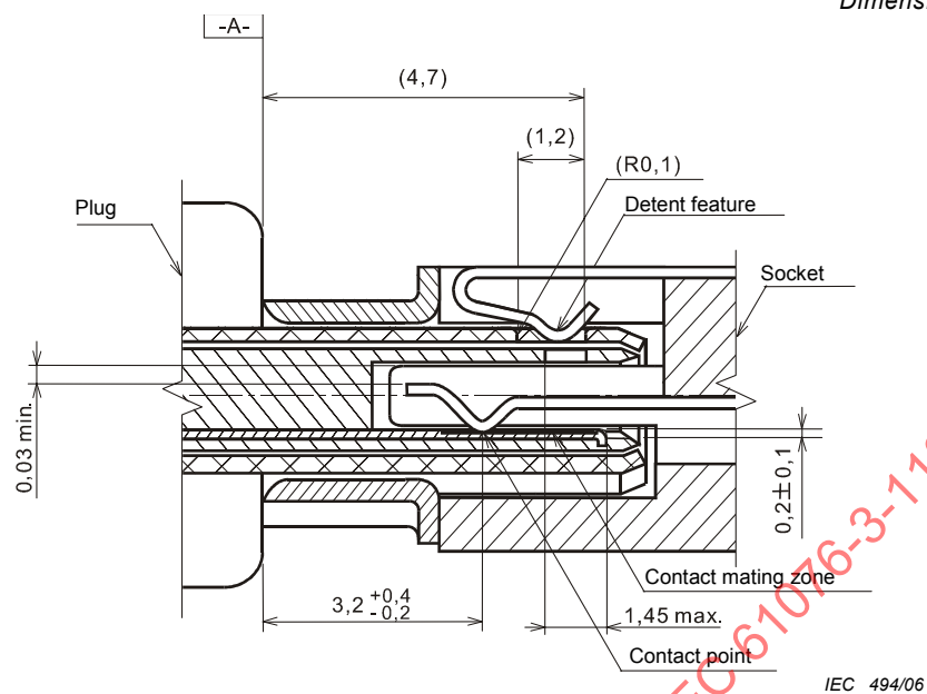
Figure 8 – Cross-section of free and fixed contacts
