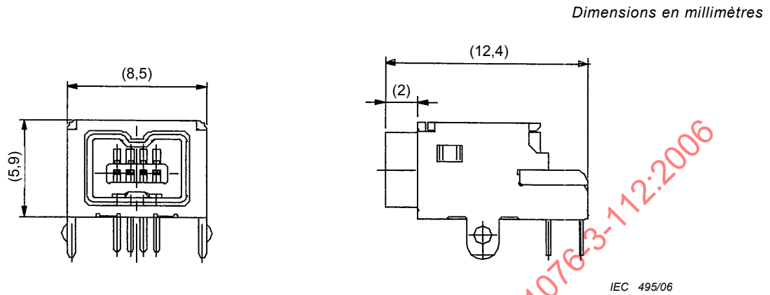
Figure 9 – Embase, modèle A
