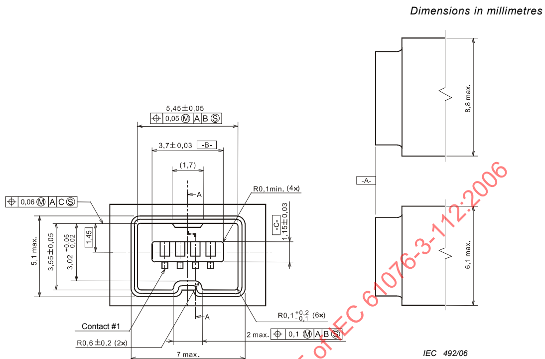
Figure 6 – Fixed connector
