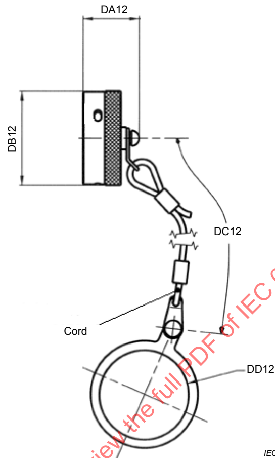
Figure 4 – Variant 11 cap for fixed connector
