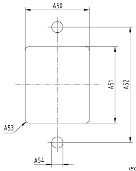
Figure 4 – Panel cut-out
