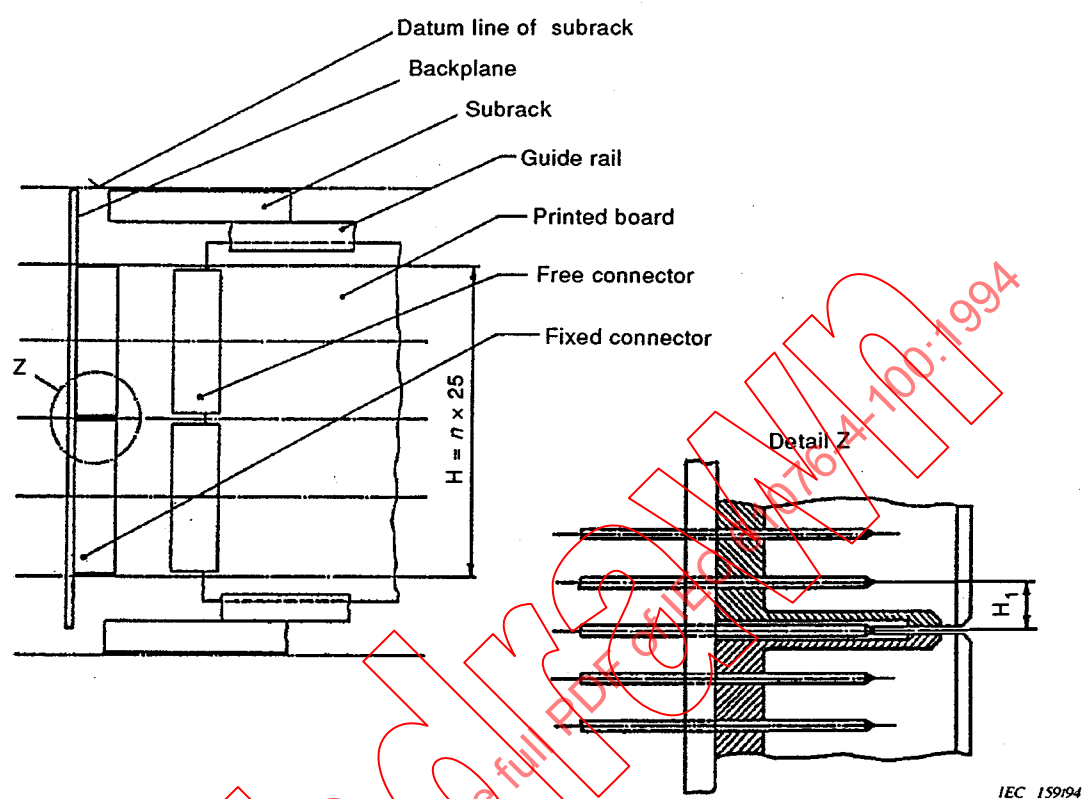
Figure 5 - Height dimensions
