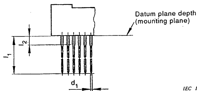
Figure 20 – Terminations
