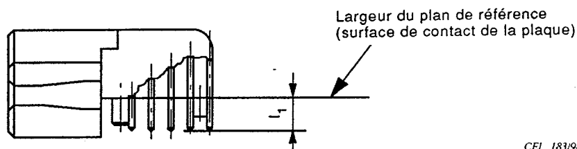
Figure 29 – Sorties
