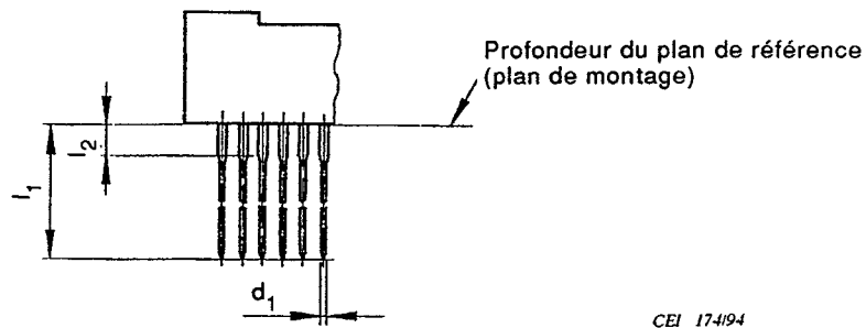
Figure 20 – Sorties
