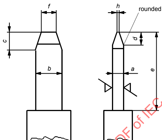
Figure 30 – Gauge dimensions
