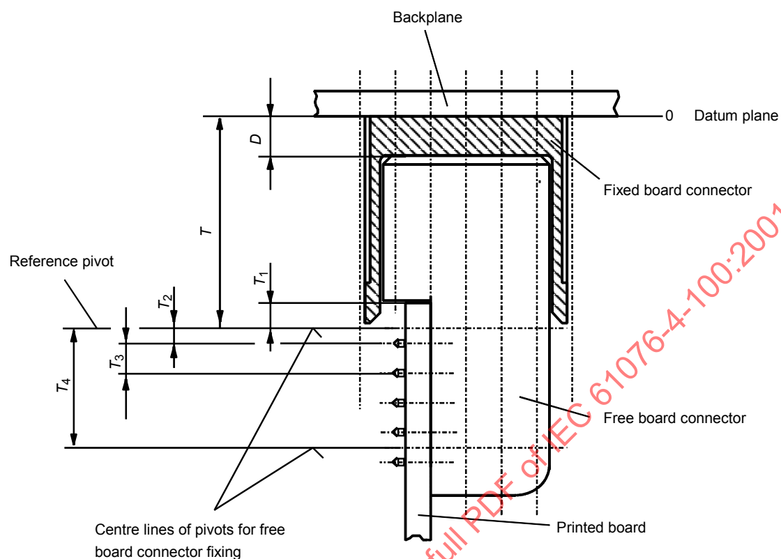
Figure 8 – Depth dimensions
