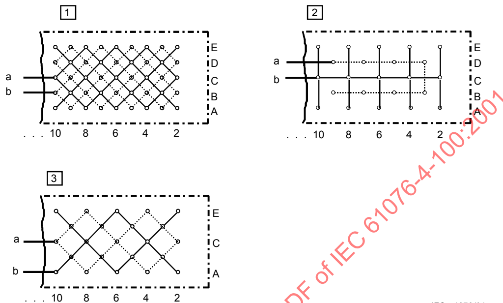
Figure 34 – Wiring of specimen
