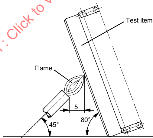
Figure 35 – Arrangement for flammability test
