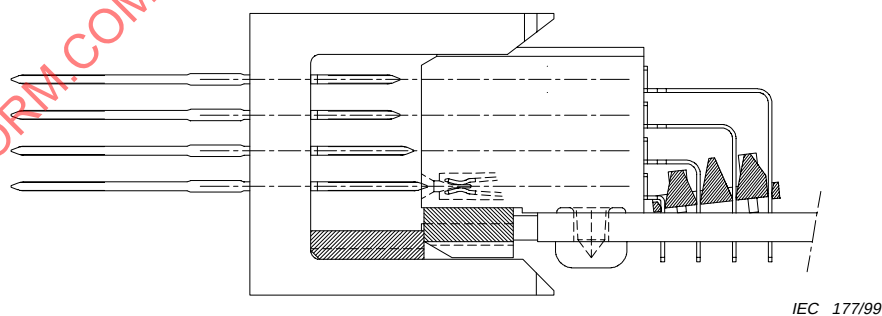
Figure 21 – Example of contact sequencing versus optional coding
