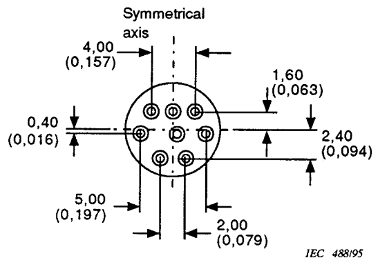
Figure 12f – Eight-contact arrangement
