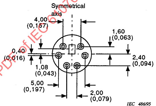
Figure 12d – Six-contact arrangement
