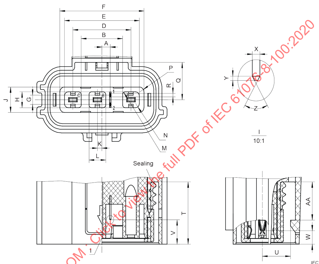
Figure 7 – 3-pole 20 A free connector
