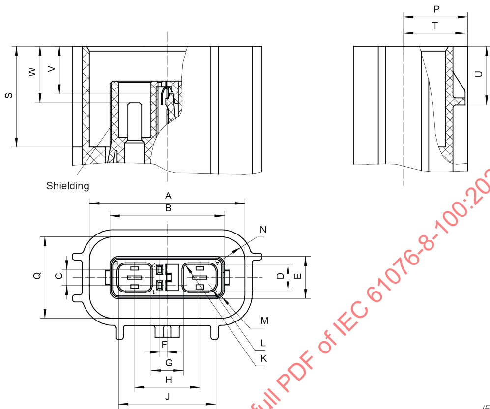
Figure 3 – 2-pole 20 A fixed connector
