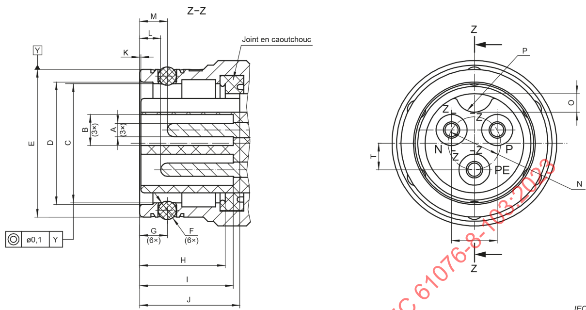
Figure 4 – Embase
