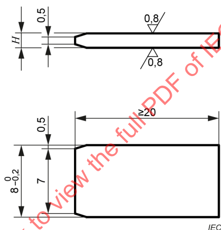
Figure 5 – Gauge for contacts
