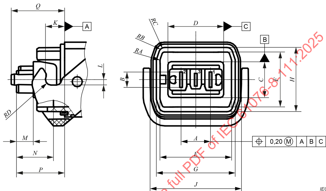
Figure 4 – Free female connector
