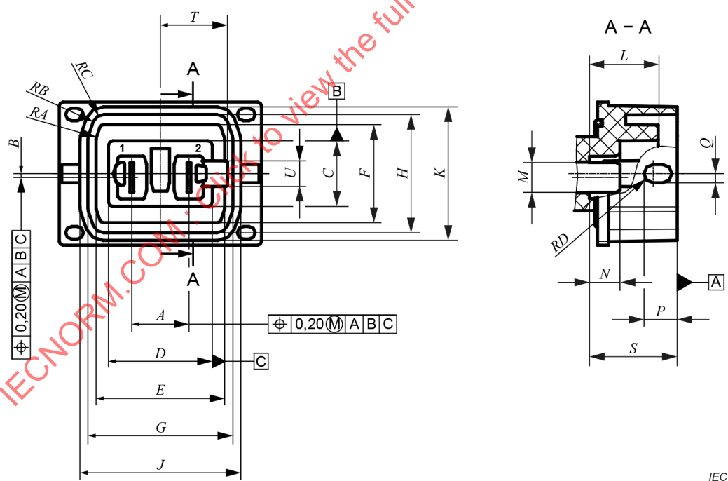
Figure 3 – Fixed male connector
