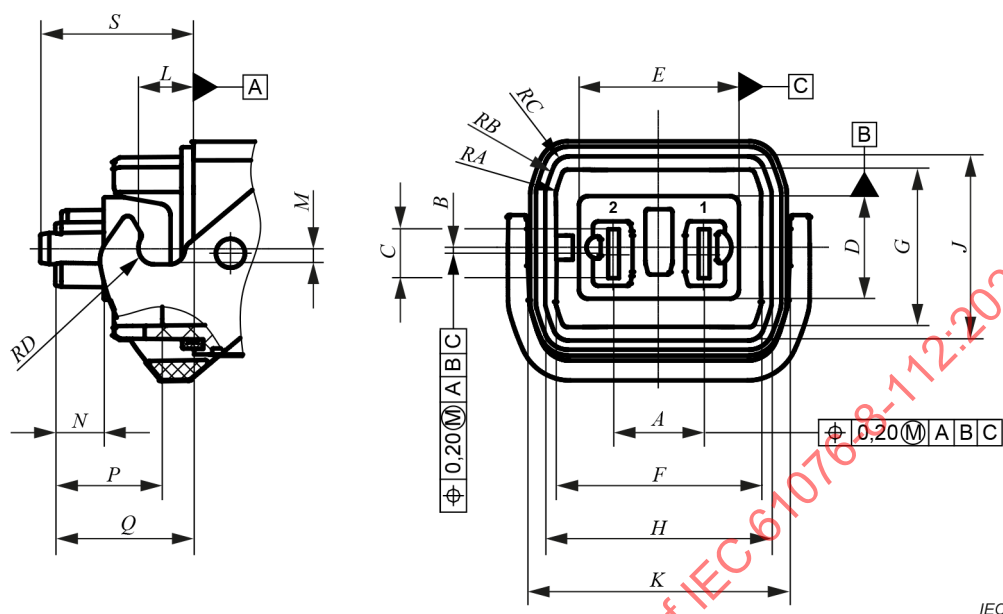
Figure 4 – Free female connector
